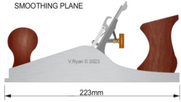
SMOOTHING PLANE
